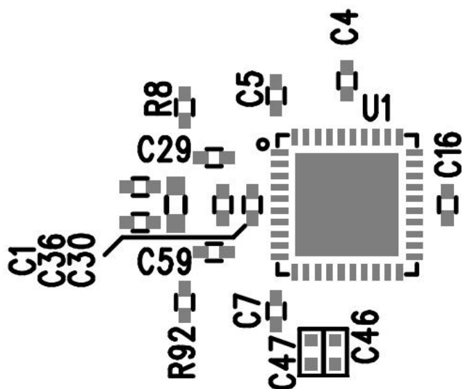
Silkscreen Top
